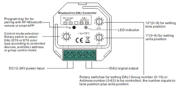
Wiring Diagram
