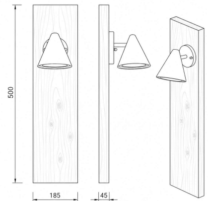
POST: 500mm (H) x 185mm (W) x 45mm (D) FITTING: 130mm (H) x 145mm (W) x 100mm (PROJ.)
