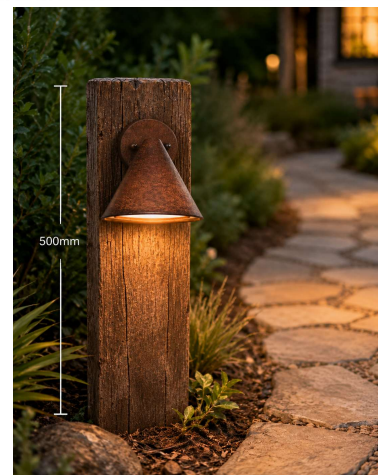
POST: 500mm (H) x 185mm (W) x 45mm (D) FITTING: 130mm (H) x 145mm (W) x 100mm (PROJ.)
